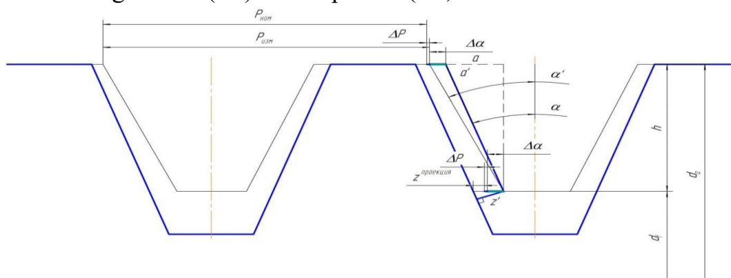
Fig. 4. Profile draft for building a dimensional chain.
