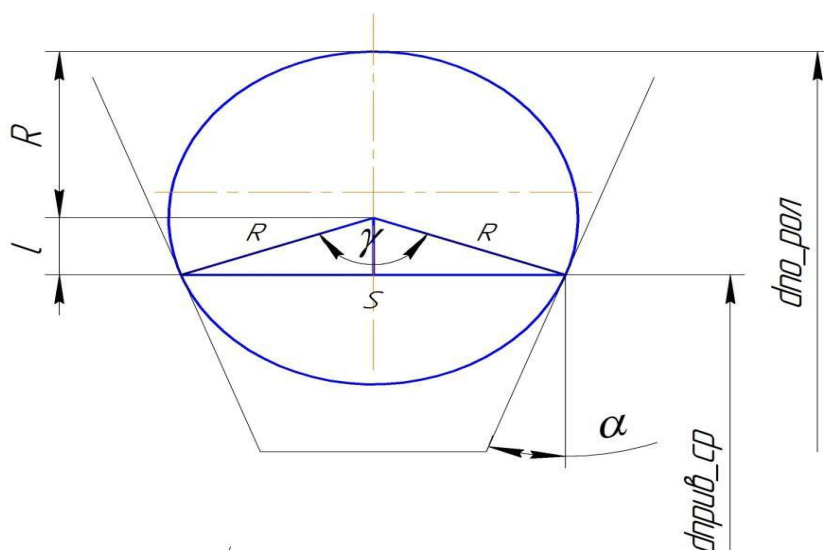
Fig. 2. Position of the measuring roller in the profile of teeth.
