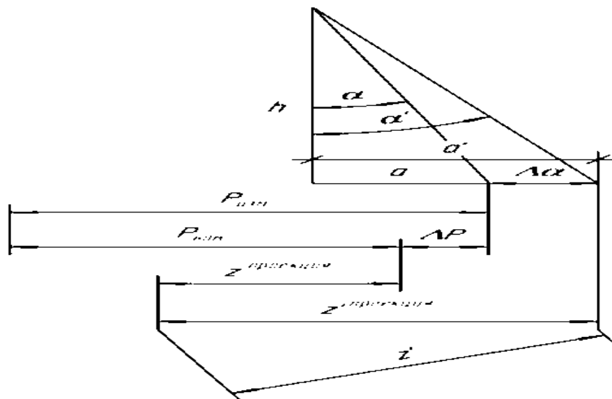
Fig. 5. Dimensional chain
