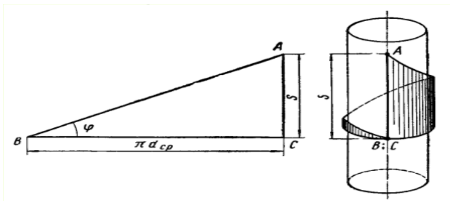
Fig 1. Formation of a helical surface
