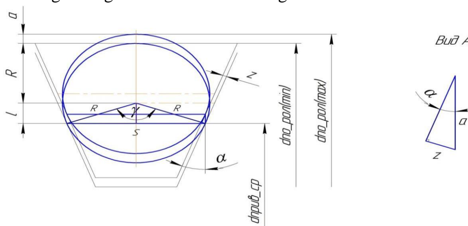
Fig.3 Determination of allowance.
