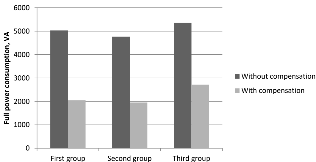
Fig. 2. The results of the experimental implementation of automatic control system for the energy intensity of mechanical engineering technological processes
