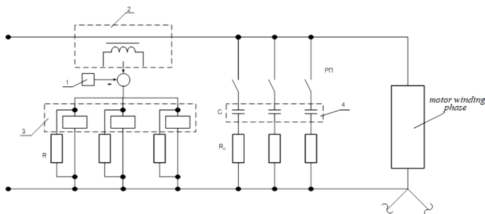
Fig. 1. Model for automatic compensation of reactive component of consumed current of asynchronous motors operating at powers lower than the rated values
